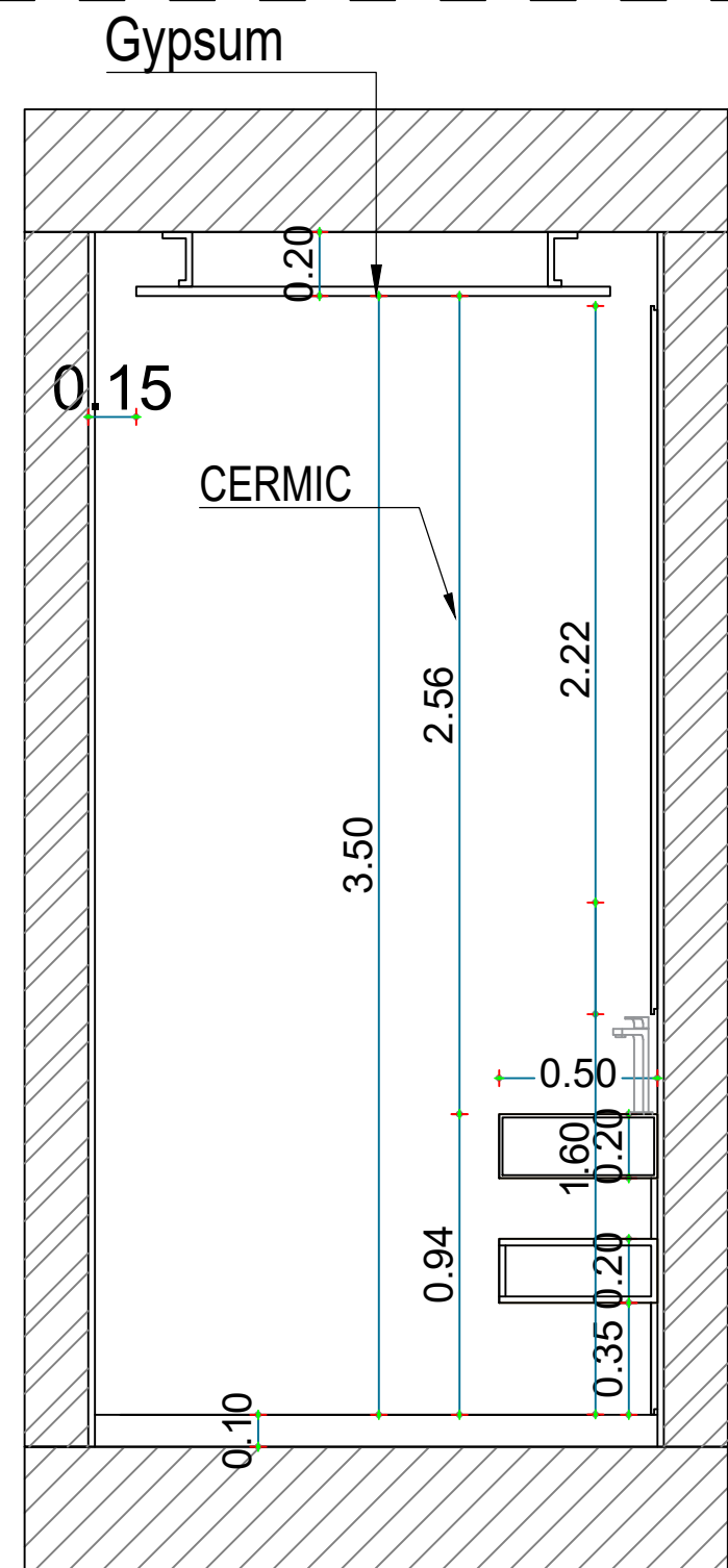
D WALL SECTION
